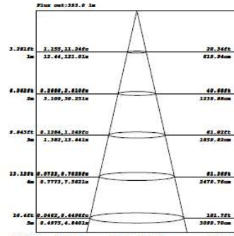
Planar Illuminance Curve
