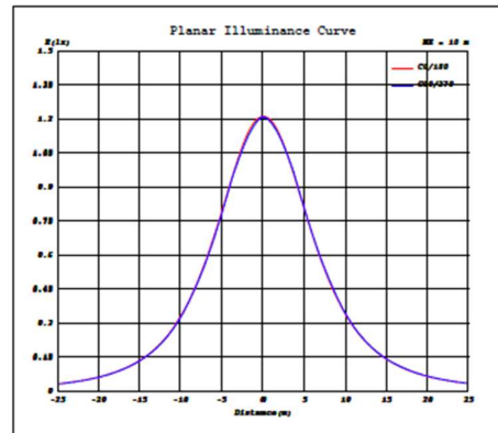
Planar Illuminance Curve
